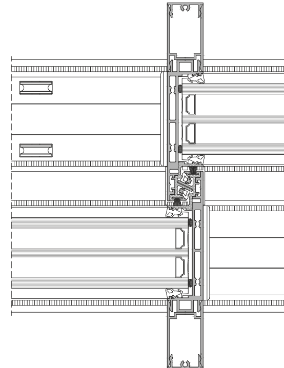
Cross-section through the leafs assembly
